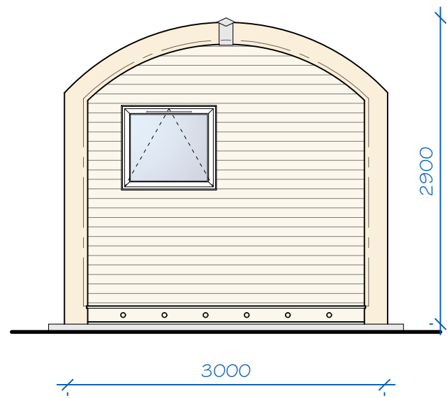
Elevation - Back Scale - 1:50 @ A3
