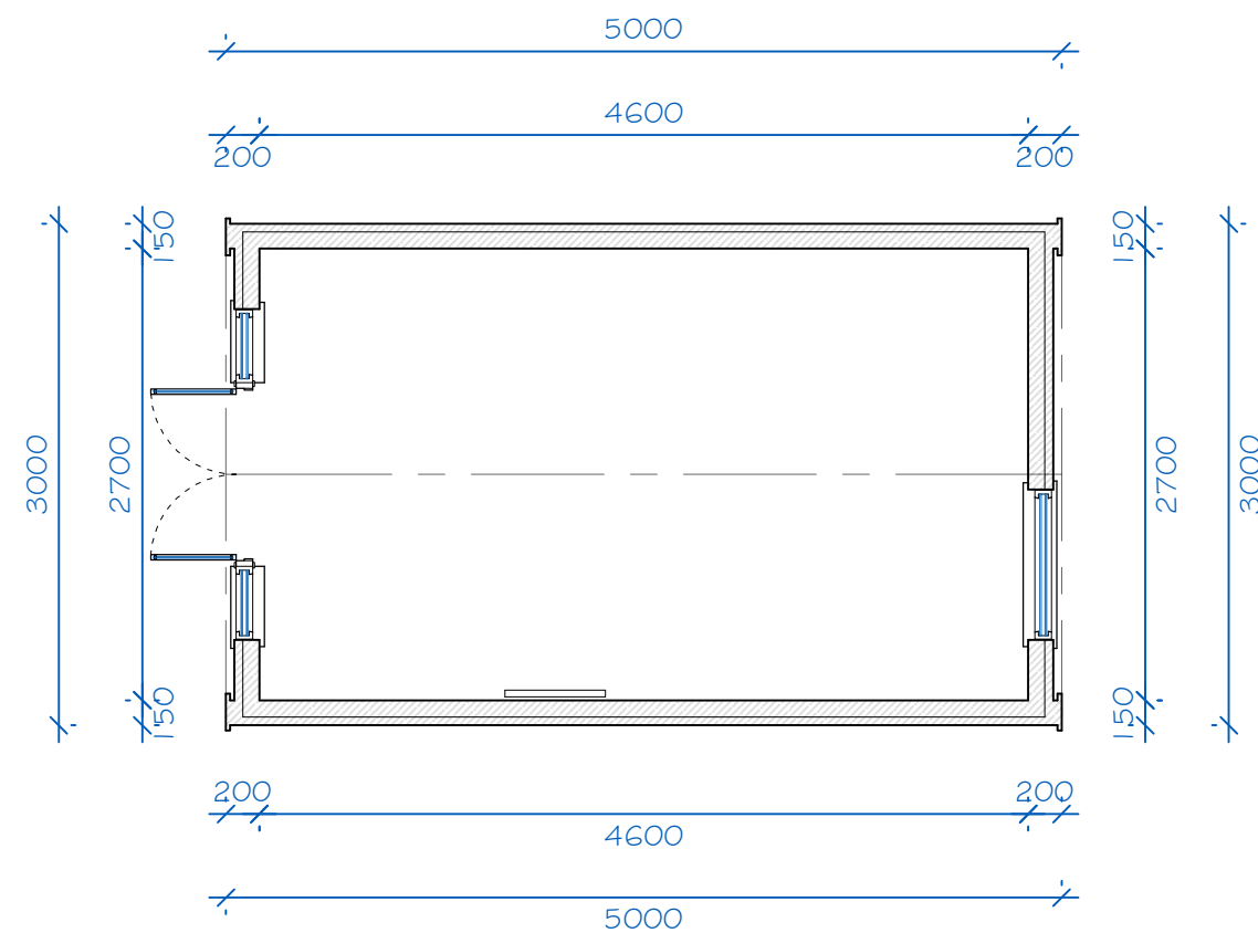
Floor Plan - Ground Scale - 1:50 @ A3
