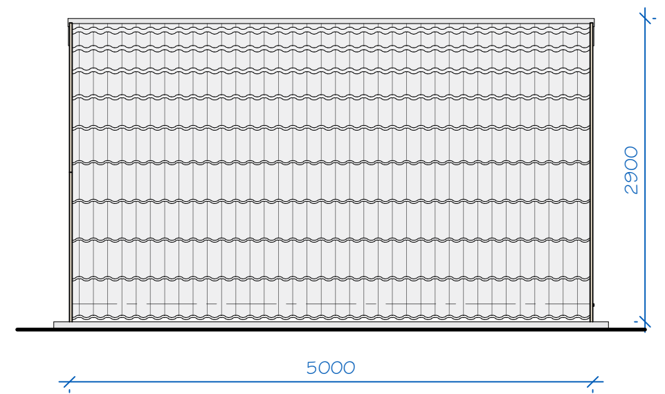
Elevation - Side Scale - 1:50 @ A3
